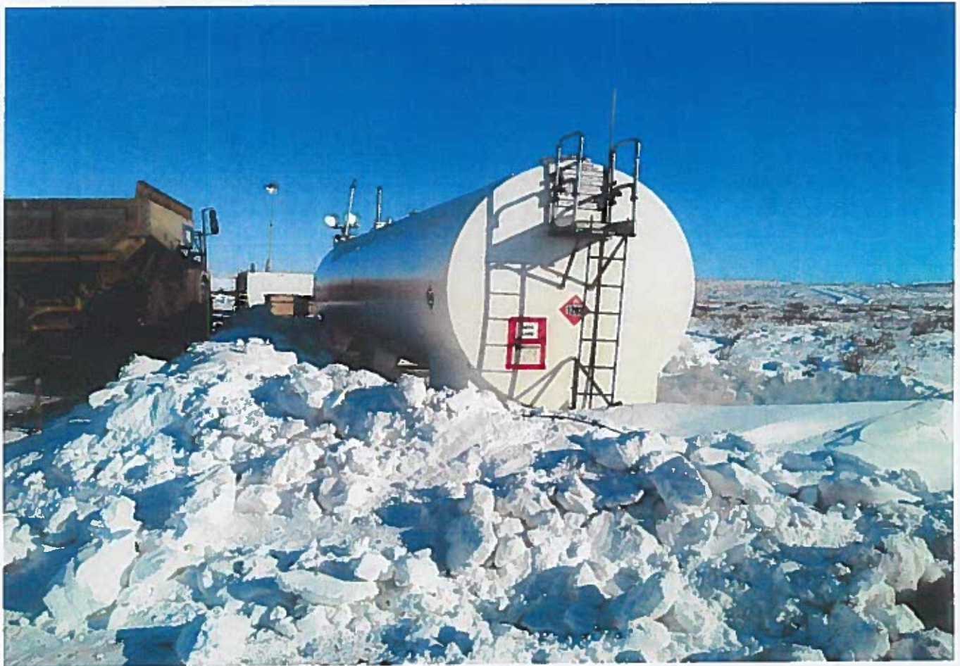
Figure 4 174 refuel area
